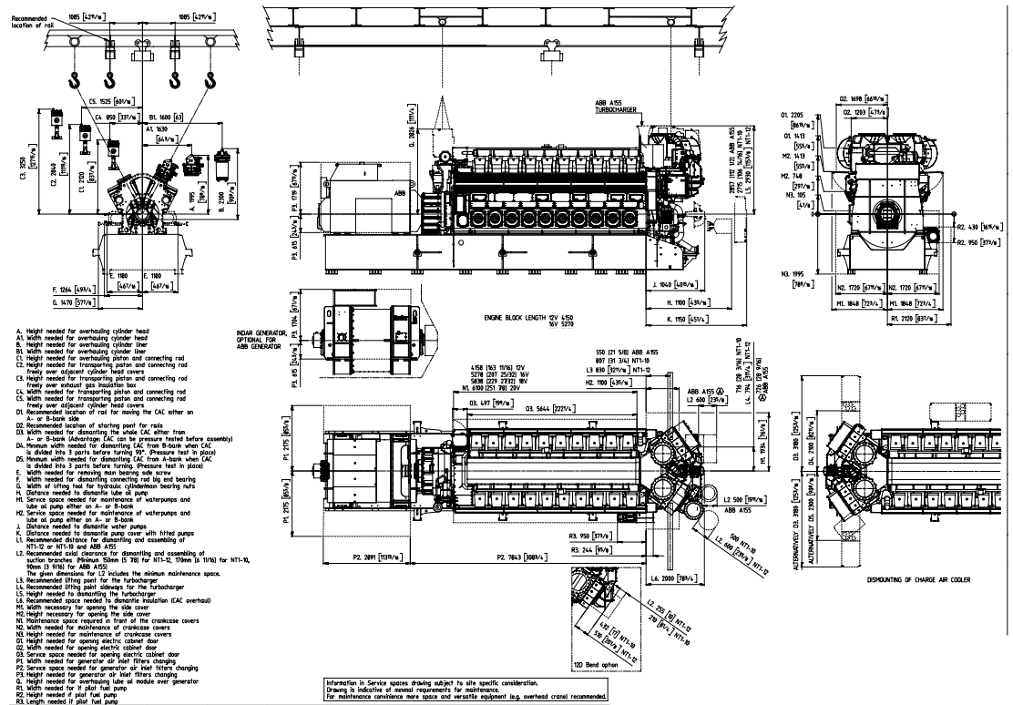
Fig 18-15 Service space requirement, genset (DAAF505533A for V-engine)
