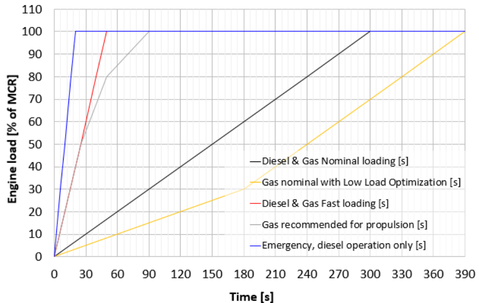
Fig 2-4 Constant speed applications
