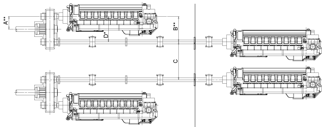
Fig 18-7 Main engine arrangement, in-line engines (DAAE086973B)
