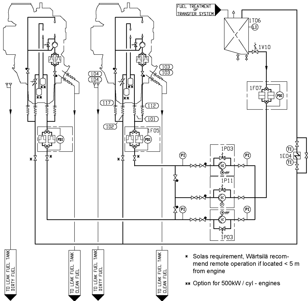
Fig 6-9 Example of fuel oil system (LFO) multiple engine installation (DAAE085364C)
