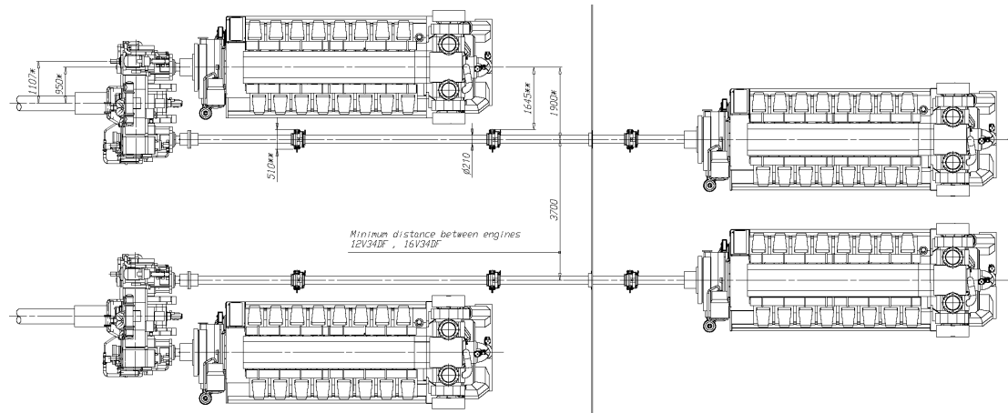
Fig 18-9 Main engine arrangement, V-engines (DAAE083977, DAAF068349)
