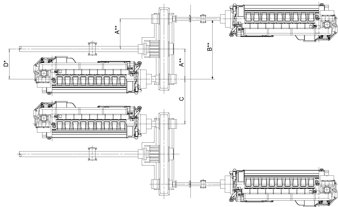
Fig 18-8 Main engine arrangement, in-line engines (DAAE086972B)
