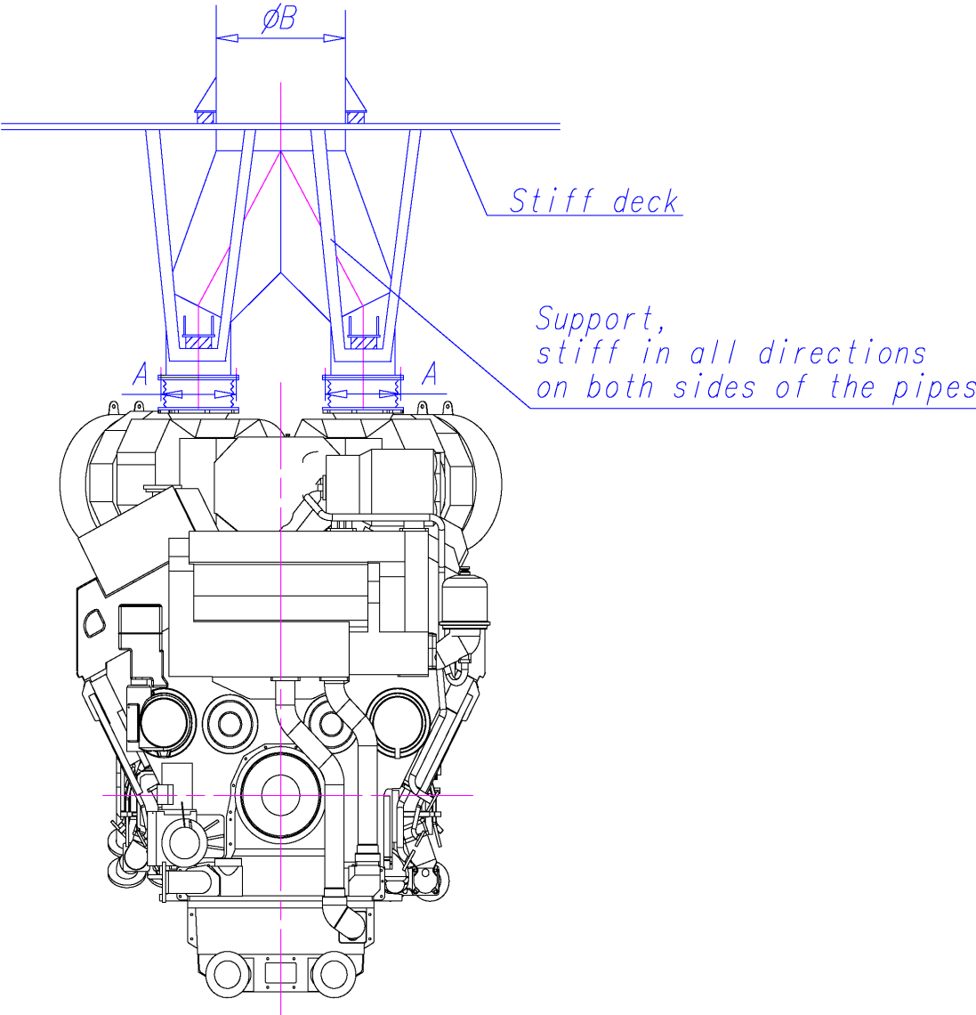
PIPE CONNECTION 501 EXHAUST GAS OUTLET ISO7005-1 PN 6
