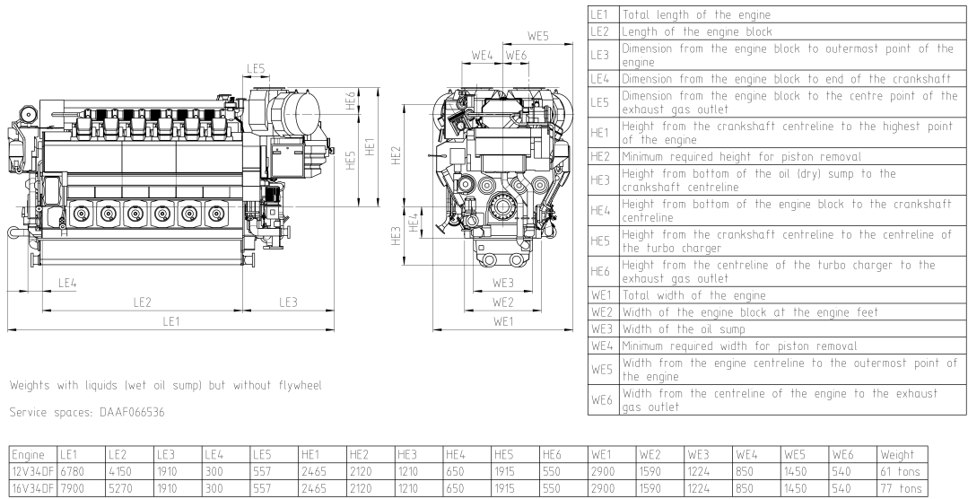
Fig 1-2 V-engines (DAAF066203A)
