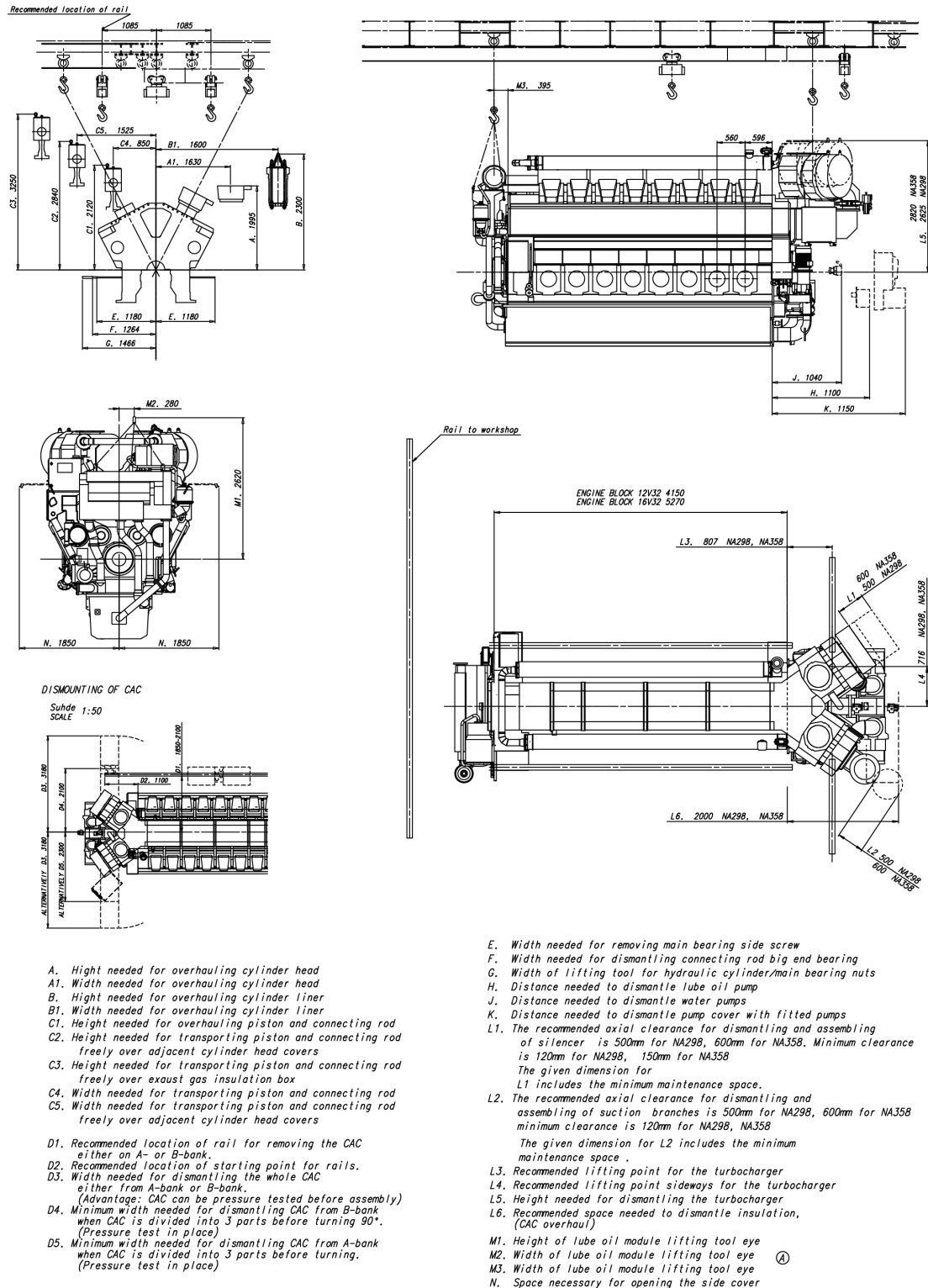
Fig 18-14 Service space requirement, turbocharger in free end (DAAF066536)
