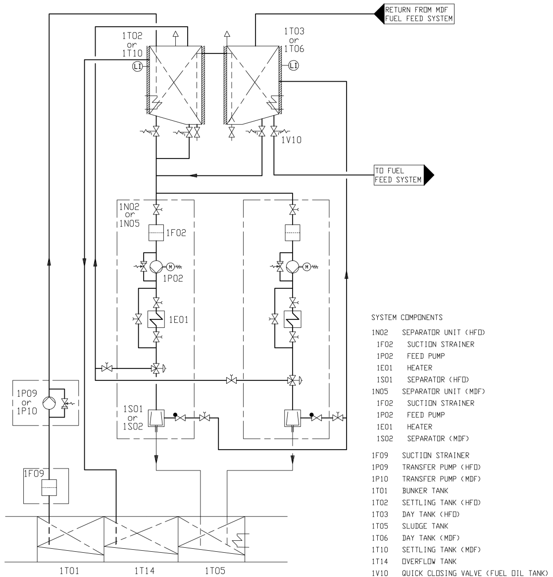
Fig 6-7 Fuel transfer and separating system (V76F6626G)
