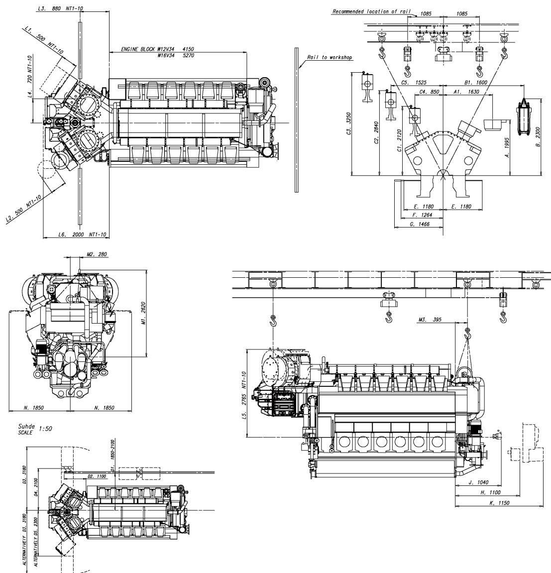
Fig 18-13 Service space requirement, turbocharger in driving end (DAAF308339)
