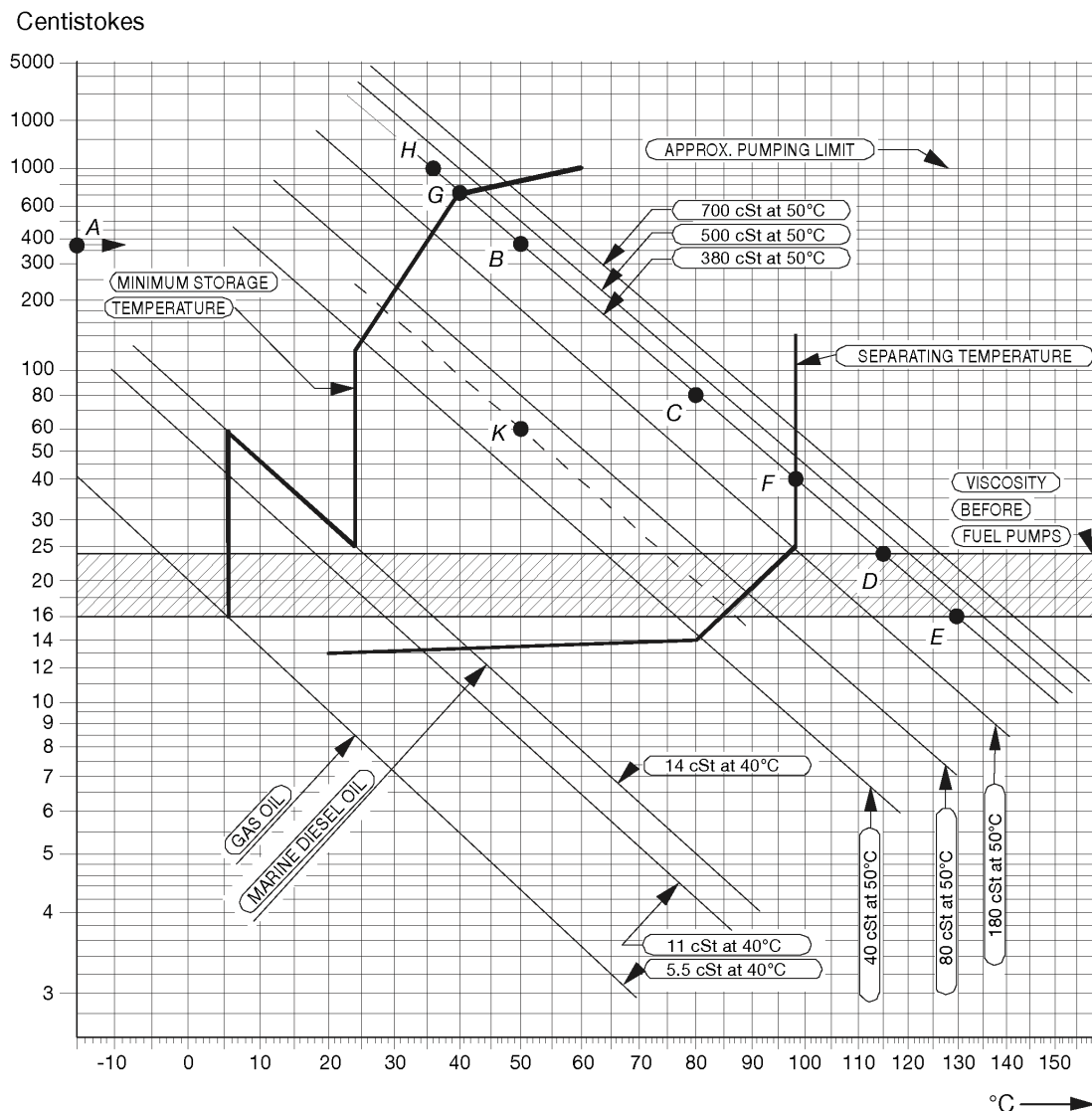
Fig 6-6 Fuel oil viscosity-temperature diagram for determining the pre-heating temperatures of fuel oils (V92G0071b)
