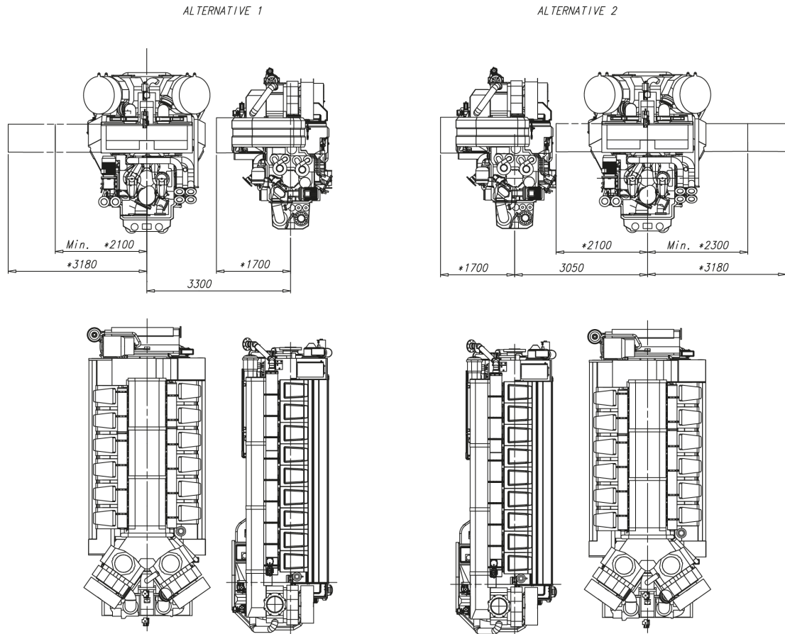
Fig 18-6 Example of father-and-son arrangement, TC in free end (DAAF073307)
