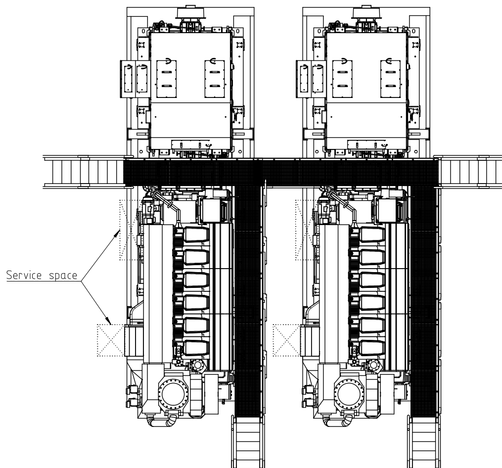
Fig 18-4 In-line engines, turbocharger in free end (DAAE082973D-2)
