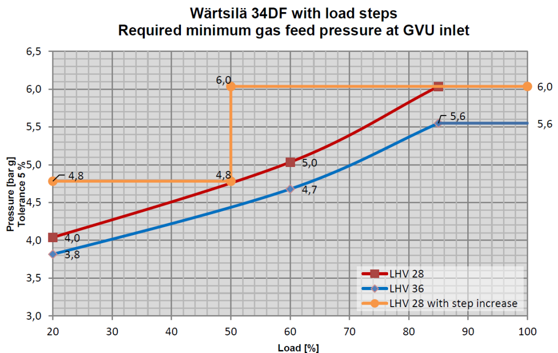
Fig 6-5 Gas feed pressure recommendation for engines including load step
