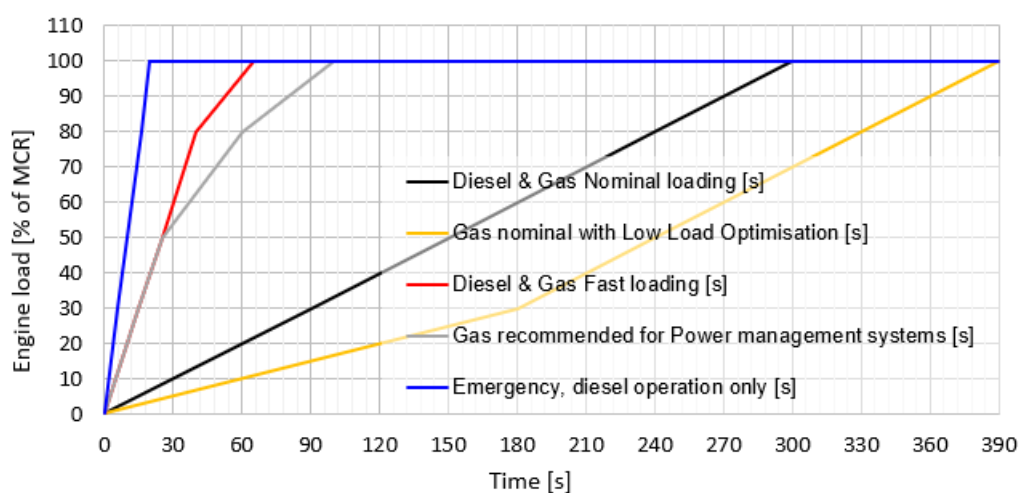
Fig 2-5 Normal Loading rate, CS 720 rpm
