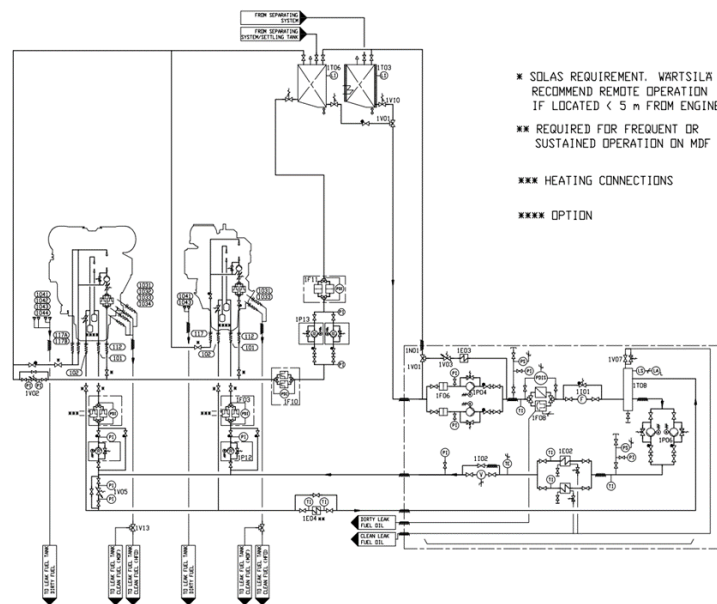
Fig 6-10 Example of FO system (HFO), multiple engine installation (DAAE085365G)
