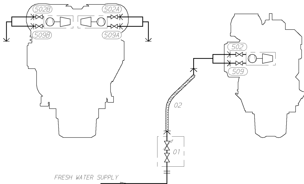
Fig 12-2 Turbocharger cleaning system (V76A2937A)
