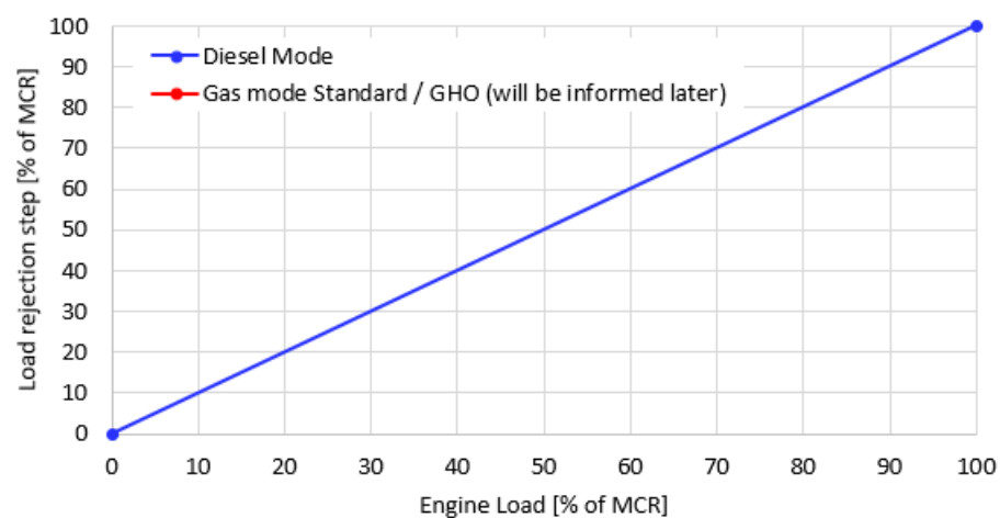
Fig 2-13 Max instant unload increase [%], Constant Speed Applications
