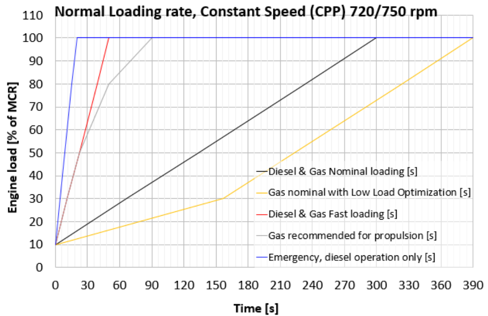
Fig 2-6 Constant speed, controllable pitch propeller (CPP)
