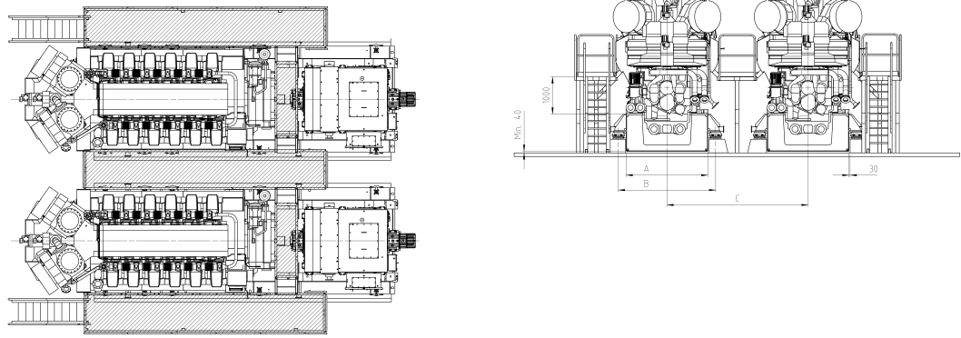
Fig 18-5 Crankshaft distances, V-engines (DAAF073293A)
