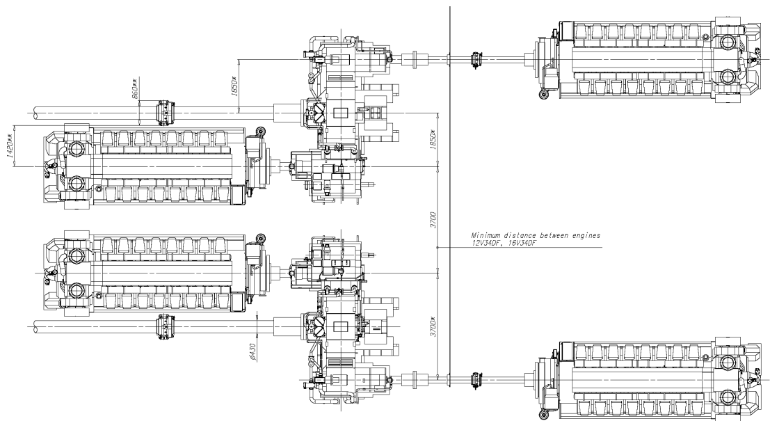
Fig 18-10 Main engine arrangement, V-engines (DAAE083975, DAAF068345)
