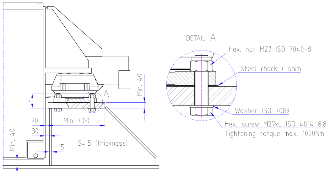
Fig 15-10 Recommended design of the generating set seating, V engines (DAAE020067C)
