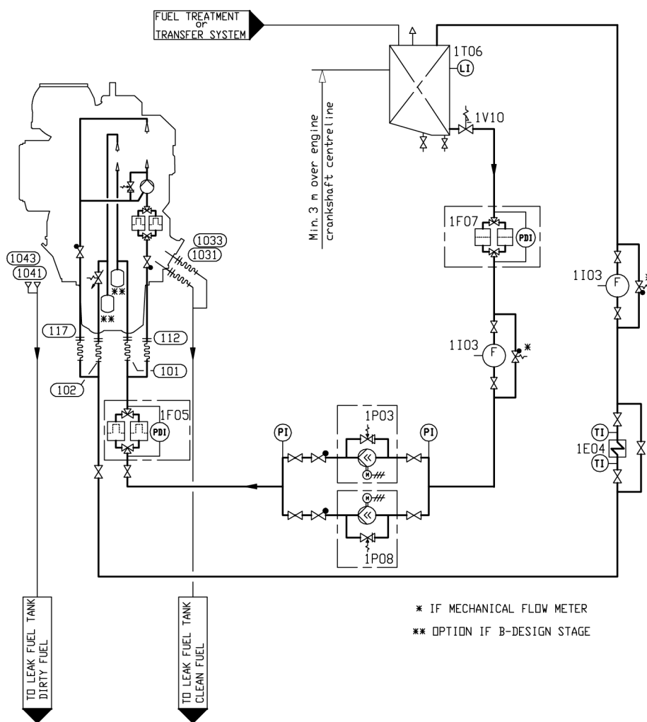
Fig 6-8 Example of fuel oil system (LFO), single engine installation (DAAE055756D)
