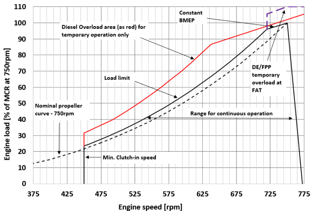
Fig 2-1 CPP operating field, diesel mode
