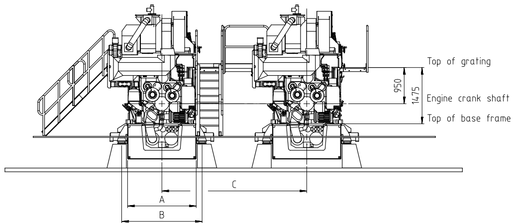
Fig 18-3 In-line engines, turbocharger in free end (DAAE082973D-1)
